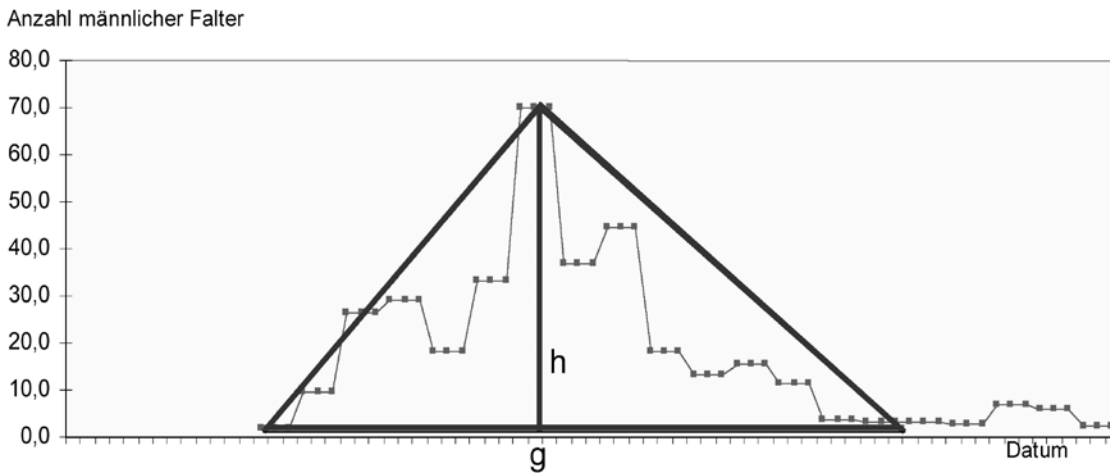
Figure 1: Maximum and total trapping values of male nun moths at locations in Saxony in years 2000, 2001 and 2003 (Bad Schandau, Falkenberg, Löbau, Muskauer Heide, Niesky, Plauen, Weißkollm) and locations in Brandenburg (Kyritz, Templin, Eberswalde, Belzig, Lübben, Wünsdorf) in the period from 1996 to 2003 (MAJUNKE et al., 2006)
